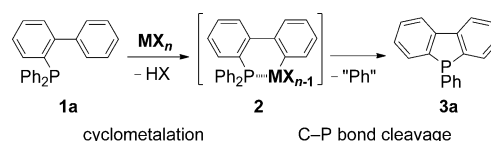
Scheme 2. Working hypothesis.
